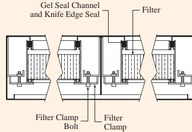
Gel Seal Style Filter Clamp Detail Typical of a Unit with Two Filters
