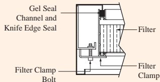
Filter Clamp Detail Typical of a Unit with One Filter
