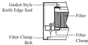
Filter Clamp Detail
